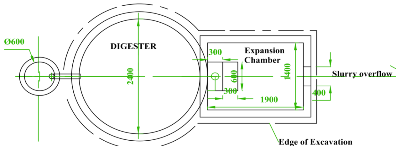
10 M3 BIO-DIGESTER PLAN
