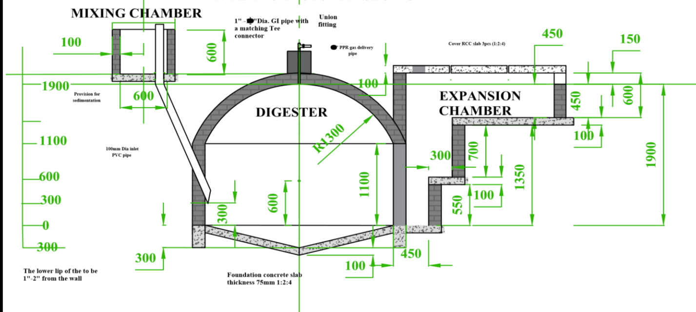
10 M3 BIO-DIGESTER SECTION
