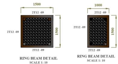
DETAIL A SCALE 1: 10
