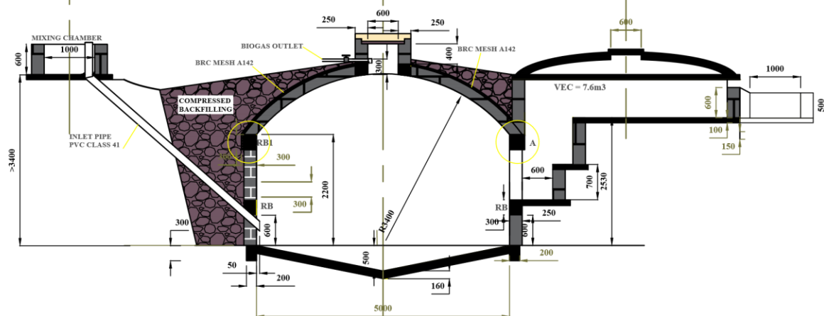
SECTIONAL VIEW 60M³ BIOGAS PLANT DESIGN SCALE 1 : 50
